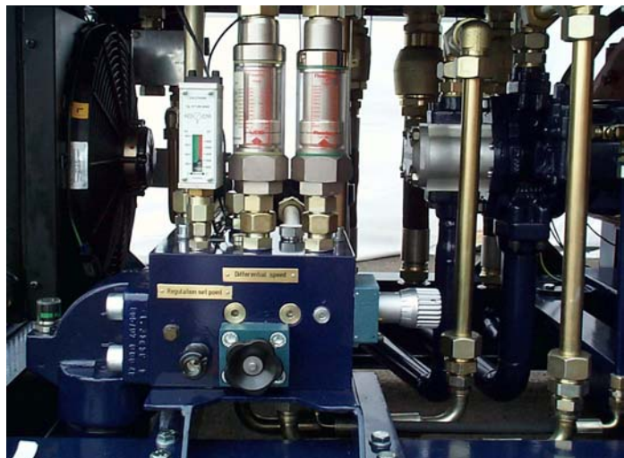
VISCOTHERM Control Block
