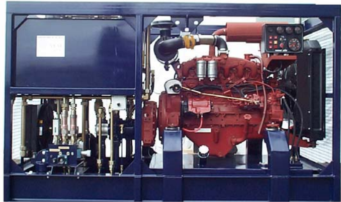
NES 402D Hydraulic Power Pack
