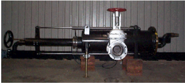
Side view of Tanksweep unit
