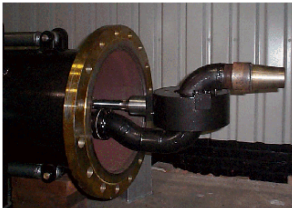
Side view with nozzle extended forward
